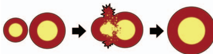
FIGURE 4 Schematic representation of core formation scenarios and how they translate into isotopic models and timescales. (A) Instantaneous core formation. In this model an age is calculated as the point in time when a fully formed planet segregated into core and silicate reservoirs. (B) Continuous core formation. The planet grows by accretion of material with a chondritic Hf/W ratio and W isotope composition. Newly accreted material is continuously mixed with W in the outer silicate portion prior to the segregation of new iron and siderophile elements (including W) into the core. Most models assume an exponentially decreasing rate of overall growth for the planet and its core. (C) Core–core mixing. Terrestrial planets appear to have formed from material that was already differentiated into silicate and metal. How much equilibration between accreted metal and the planet's silicate reservoir occurs [an explicit requirement in calculating an age with model (B) ] is not well understood at present. The net result, if calculated with continuous core formation and equilibration as in model (B) , is that the rate of growth of the planet appears faster than it really was.
