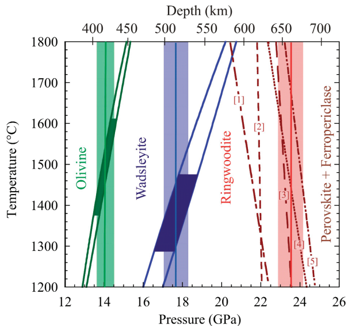
FIGURE 3 Pressure–temperature slopes for transition zone phase transformations compared to average discontinuity depths (vertical solid lines) and global topography (vertical shaded regions) of the 410 (green), 520 (blue) and 660 km (red) discontinuities. Double curves for the olivine–wadsleyite and wadsleyite–ringwoodite transformations indicate the depth intervals where transforming (\text{Mg,Fe})_2\text{SiO}_4 solid solutions coexist (Frost 2003). These curves are shaded to indicate temperature ranges compatible with global discontinuity topography. The figure also shows individual curves for the \text{Mg}_2\text{SiO}_4 ringwoodite to perovskite + periclase reaction from different studies: [1] Irifune et al. (1998), [2] Katsura et al. (2003), [3] Fei et al. 2004, [4] Ito and Takahashi (1989) and [5] Shim et al. (2001).
