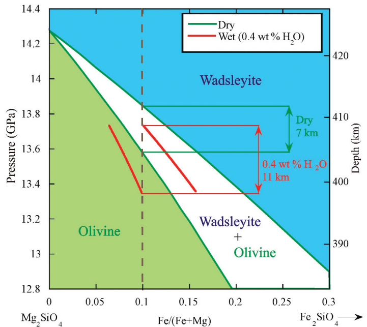
FIGURE 4 The olivine-wadsleyite transformation in the Mg 2 SiO 4 -Fe 2 SiO 4 system calculated at 1400°C under dry conditions and with 0.4 wt% H 2 O (Frost and Dolejš 2007), which is the H 2 O content required to saturate olivine at these conditions. The downward displacement of the two-phase region in the hydrous system is shown by the red curves. The vertical dashed line shows a typical mantle Fe/(Fe+Mg) ratio of 0.1. The dry transition is approximately 7 km wide, while the addition of H 2 O broadens the transition at these conditions to a maximum of 11 km.
