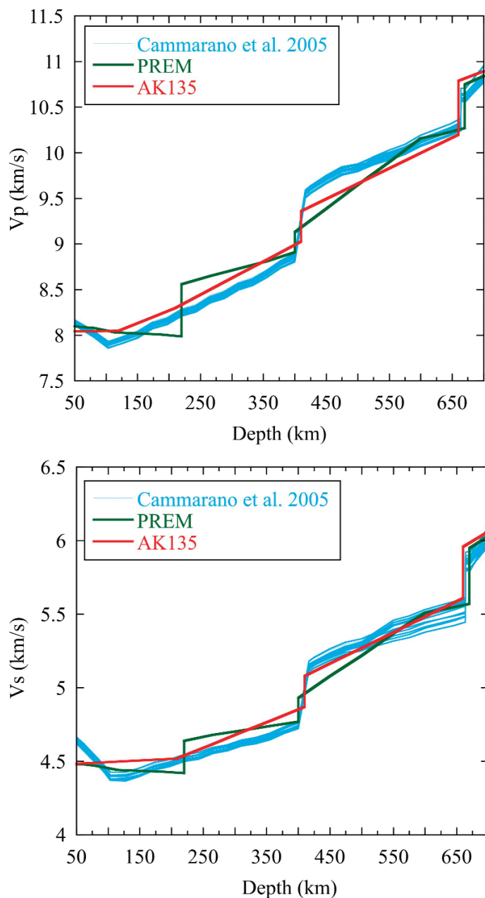
FIGURE 2 Seismic reference models PREM, AK135 and those of Cammarano et al. (2005) showing S- and P-wave velocity structure in the upper mantle and transition zone. The numerous reference models by Cammarano et al. (2005) were obtained by fitting similar global seismic data, as used in PREM, for example, to 1-D velocity models calculated for a pyrolite mineral assemblage by adjusting mineral elastic properties within the range of their uncertainties. The different models therefore arise from the use of slightly different sets of mineral properties, although all models still fit the same seismic data.
