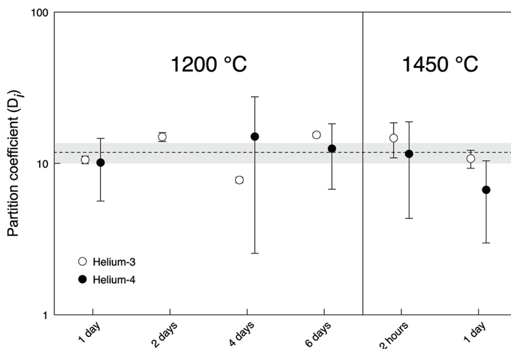
Figure 2 Metal-silicate (liquid-solid) partition coefficients for He. The dashed line shows the average partition coefficient D_{\text{He}} value of 11.8 ( n = 11 ). The shaded area defines the two standard error of the mean (2 se) of 1.8. Data for the two-hour experiment are excluded and the ^4\text{He} partition coefficient for the two-day experiment is missing. Uncertainties include only gas concentration uncertainties. Error bars are 2 sd.
