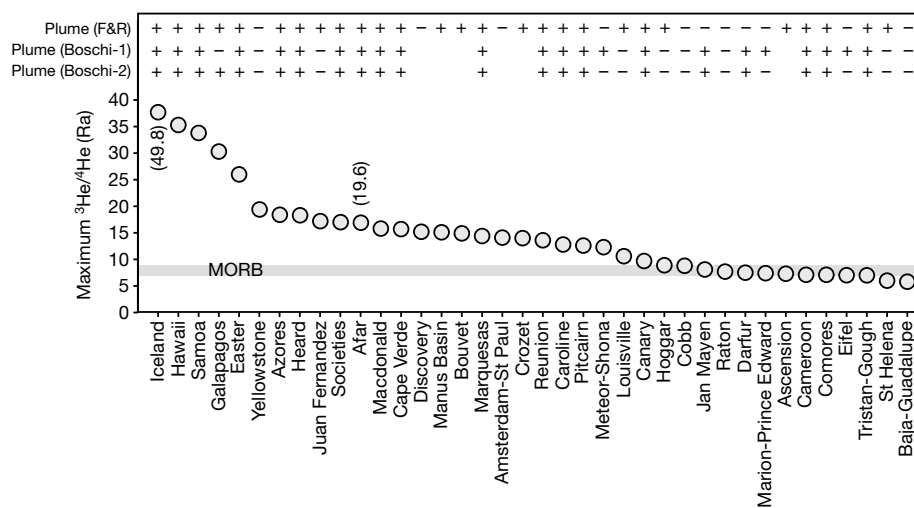
Figure 1 | The maximum ^3\text{He}/^4\text{He} values at 38 hotspots organized in order of decreasing maximum ^3\text{He}/^4\text{He} . See Supplementary Table 1.
