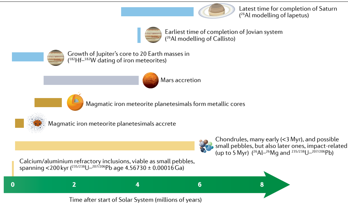
Fig. 2 | Chronology of the earliest Solar System, as determined from various isotopic systems. The oldest Solar System solids are the calcium–aluminium refractory inclusions (CAIs) forming at <math><200\text{ kyr}</math> after the start of the Solar System. These were followed shortly after by the formation of chondrules that persisted for several million years. The timing of planetesimal accretion (<math>\sim 300\text{--}500\text{ kyr}</math>) and differentiation (<math>\sim 800\text{ kyr}</math> to 1.5 Myr) is inferred from the age of iron meteorites. Mars's accretion occurred early, probably within
