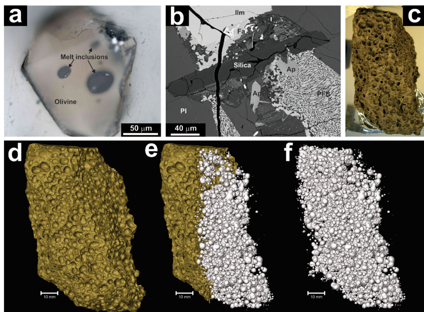
Figure 2. Evidence for volatiles in lunar samples. (a) Visible-light photomicrograph of olivine-hosted melt inclusions in 74220 after rehomogenization. (b) Back-scattered electron image of apatites within high-Ti mare basalt 10044,33. Phase abbreviations are as follows: Ap—apatite, Fa—fayalite, Ilm—ilmenite, PFB—pyroxferroite breakdown products, Pl—plagioclase. (c) Visible light image of Apollo sample 15556,215 (354 g; FOV = 10 cm long dimension), a vesicular lunar basalt sample from the Apollo 15 mission. (d–f) Three different images from an X-ray Computed Tomography (XCT) scan of vesicular lunar basalt sample 15556,215 (prepared by Scott Eckley). (d) An XCT isosurface view of the exterior of sample 15556,215. (e) An XCT image of both the isosurface view of the exterior (left side, in gold), as well as an isosurface view of void spaces within 15556,215 (right side, in white). (f) An XCT isosurface view of the void spaces within sample 15556,215.
