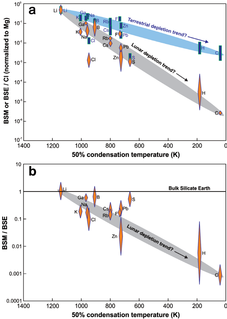
Figure 6. Abundances of select volatile elements in BSM, BSE, and CI chondrite as a function of 50% condensation temperature at 10^{-4} bars (Lodders 2003). Volatile depletion trends for the Earth ( blue ) and Moon ( gray ) are estimated with an envelope that has a slope defined by Li and C abundances (a) Abundances of select volatile elements in BSE ( blue symbols ) and BSM ( orange symbols ), normalized to Mg and CI chondrite (after McDonough and Sun 1995) using data from Table 2. (b) Abundances of select volatile elements in BSM normalized to BSE.
