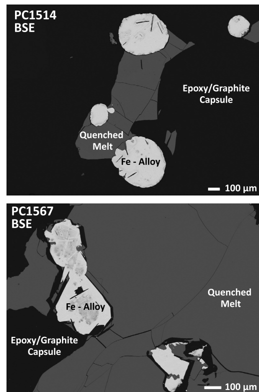
Fig. 1. Backscattered electron (BSE) images of two experiments from this study. Black regions are epoxy or graphite from the sample capsule. Gray regions are quenched melt and the bright regions are Fe–Si–C-alloy. The patchy discoloration on the surface of some of the alloys is oxidation from polishing and black inclusions in the alloys are graphite from the sample capsule.
