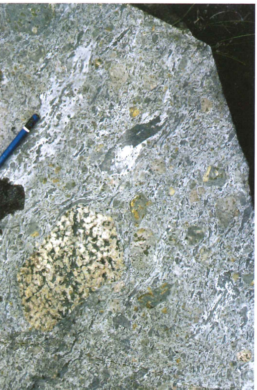
An ignimbrite from Oppkuven in Krokskogen, containing large clasts (lithic fragments) that have been torn from the country rock during the explosion. A well-defined layering or striping within the rock represents compressed pumice fragments (dark grey) that were formed during the explosive eruptions of the “Oppkuven volcano” that occurred during formation of the Oppkuven caldera. The presence of fragments of this size within the ignimbrite indicates that we are quite close to the site of the eruption. The pencil is about 8 cm long. (Photo: B. T. Larsen)
