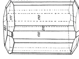
Fig. 66. Vesuvian, \{001\} , \{100\} , \{110\} , \{210\} , \{111\} , \{101\} , Sata, Konnerudkollen.
