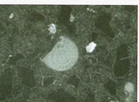
Thin section of a fusilinid viewed through a microscope. From the Tanum Formation on Jeløya near Moss. The fossil is 0.5 mm across. (Photo: S. Olausen)
